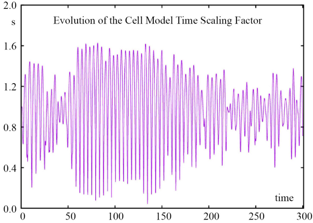
Fig. 2. Evolution of the time-scaling factor s for the Toy Model cell model for the initial 300 000 fourth-order Runge-Kutta timesteps of 0.001 using \dot{s} = p_s ; \dot{p}_s = (p_x^2 + p_y^2)/s^3 - (1/s)
