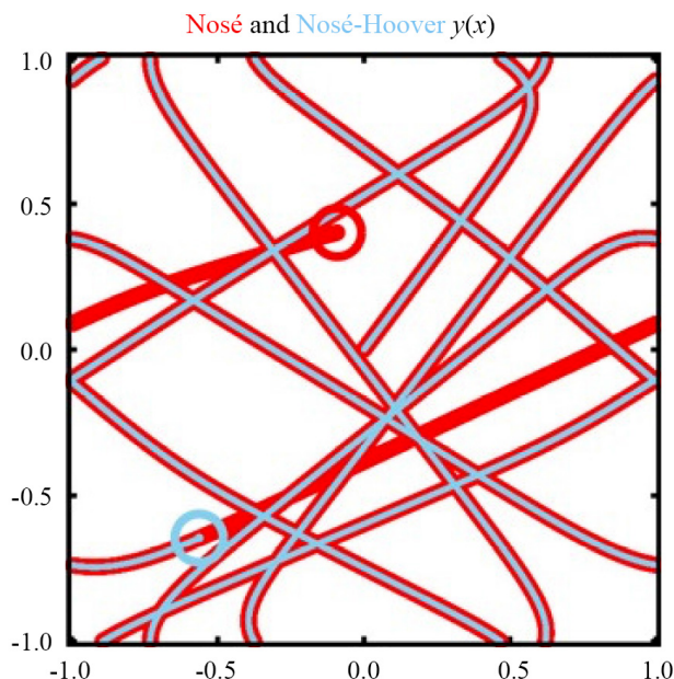
Fig. 3. Evolution of the cell model coordinates (x, y) from Nosé's Hamiltonian (red), and concluding at the open red circle just above the origin are compared to those from the Nosé-Hoover motion equations (blue, and ceasing at the blue open circle at lower left). The two approaches follow identical trajectories , but at different rates . Here the results of 20 000 fourth-order Runge-Kutta timesteps are displayed for both sets of motion equations with initial conditions (x, y, s, p_x, p_y, p_s = \zeta) = (0, 0, 1, 0.6, 0.8, 0)
