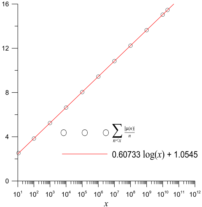
Fig. 1. The plot of values of \sum_{n < x} \frac{|\mu(n)|}{n} captured at x = 10, 100, \dots, 10^{10}, 2 \times 10^{10} . For the fit the first two values of x were skipped
