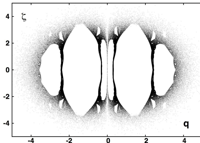
Fig. 1. The p = 0 cross section of the chaotic sea for the Nosé-Hoover harmonic oscillator. 502 924 crossings of the plane are shown. The fourth-order Runge-Kutta integration used a timestep dt = 0.0001 . A point was plotted whenever the product p_{old}p_{new} was negative
