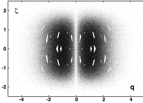
Fig. 2. The p = 0 cross section of the chaotic sea for an oscillator governed by Brańka, Kowalik, and Wojciechowski's choice of the motion equation, \dot{q} = \dot{p} = -q - \zeta^3 p ; \dot{\zeta} = p^2 - 1 . 20 billion timesteps, with dt = 0.0001 , resulted in 636 590 crossings of the p = 0 section, using the integration procedure of Fig. 1
