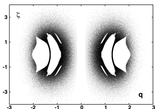
Fig. 3. p = 0 cross section for a singly-thermostated quartic oscillator, with motion equations \ddot{q} = \dot{p} = -q^3 - \zeta p^3 ; \dot{\zeta} = p^4 - 3p^2 . Runge-Kutta integration as in Figures 1 and 2 with 503 709 crossings of the p = 0 plane. Several hundred singly-thermostated attempts failed to obtain canonical ergodicity for the quartic oscillator
