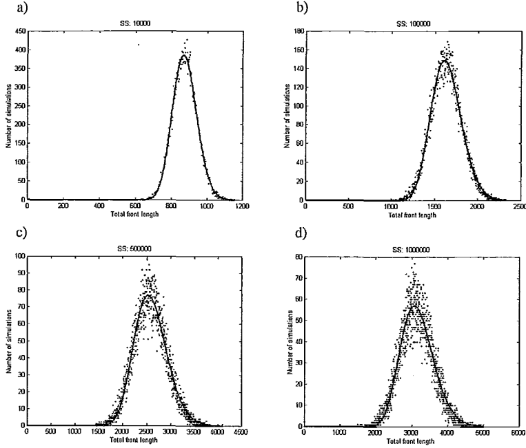
Fig. 3. Tendency towards lognormality in size is shown for the total length of the multilane against the number of simulation steps SS = 10^4, 10^5, 5 \times 10^5, 10^6 , from top left to bottom right, respectively (the linear lattice size is taken at L = 200 ). The corresponding (\sigma, \nu) pairs are as follows: 0.077, 6.774; 0.107, 7.399; 0.133, 7.852; 0.147, 8.051, cf. the mathematical form of logarithmic Gaussian, given in Section 3.
