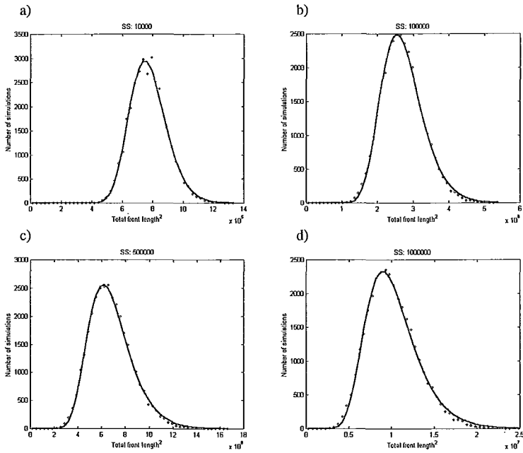
Fig. 4. Same as in Fig. 3 is shown for the square of the total length of the multilane against the number of simulation steps SS = 10^4, 10^5, 5 \times 10^5, 10^6 , from top left to bottom right, respectively ( L = 200 ). The corresponding (\sigma, \nu) pairs are as follows: 0.156, 13.551; 0.216, 14.799; 0.267, 15.705; 0.296, 16.103.
