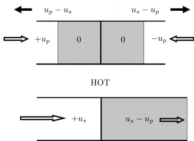
Fig. 1. Shockwave generation. In the upper view two mirror-image cold fluids collide with velocities \pm u_p generating a pair of shockwaves, moving at velocities \pm(u_s - u_p) as they convert the cold moving fluid to its hot (shaded grey) motionless shocked state. The lower view shows a stationary shockwave: cold fluid approaches from the left, encounters the hot slower fluid, and slows, [u_s \rightarrow u_s - u_p] converting a portion of its kinetic energy to internal energy. The simulations discussed in the text and illustrated in the other Figures correspond to the geometry of the upper view, with periodic boundary conditions in both the x and y directions
