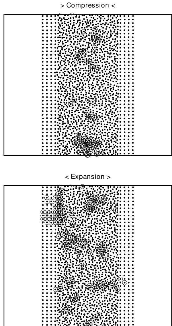
Fig. 4. Particle positions at time 10.0, after 1000 timesteps with \Delta t = 0.01 . The motion is precisely reversed at times of 30, 70, 110, . . . . The kinetic energy reaches a minimum at a time of 12.3, corresponding to maximum compression. In the reversed expanding motion the minimum occurs at a time of 47.7. After four periodic reference cycles, each of duration 80, the nearby satellite trajectory has converged to machine accuracy. The larger open circles in the top view enclose the 101 particles making above-average contributions to \lambda_1^{\text{forward}} . The more numerous particles (212) making above-average contributions in the reversed motion are shown in the bottom view with open circles
