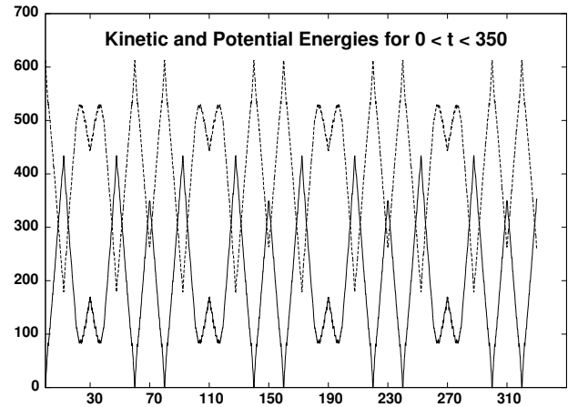
Fig. 2. Kinetic (dashes) and Potential energies for a 1600-particle bit-reversible system as functions of time. Maximum compression, about twofold, occurs at a time of 12.3. All the velocities are precisely reversed at times of \{30, 70, 110, 150, \dots\} so that maximum compression occurs again at time (60 - 12.3 = 47.7) . The velocity reversal times correspond to the tick marks on the abscissa
